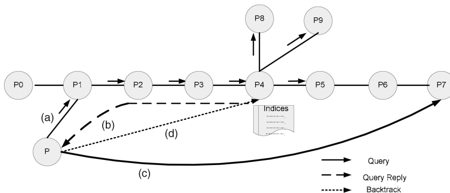
Fig. 9. Backtrack Clearing: (a) Node P sends out a query. (b) Node P4 responses back the query reply generated from cache index. (c) Based on the query reply, node P requests file from node P7. (d) If the file is not available, a backtracking clearing message is sent back from node P to node P4.
