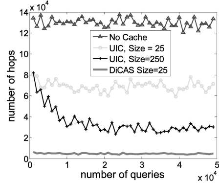
Fig. 12. Traffic comparison of UIC versus DiCAS.
