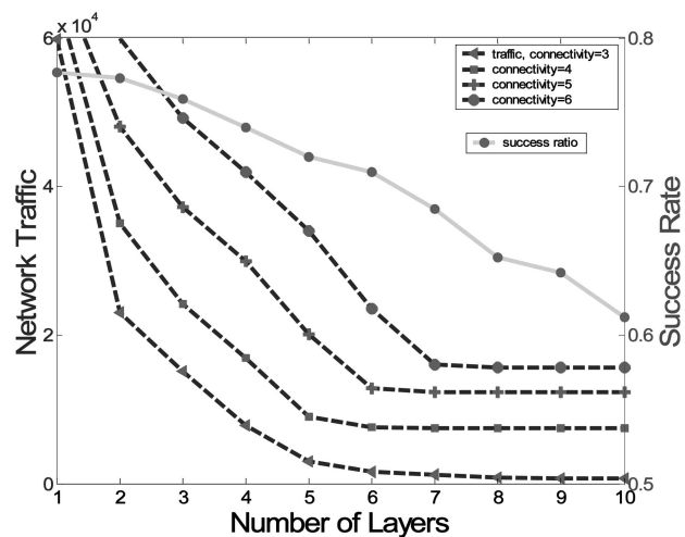
Fig. 15. Comparison for different number of layers.
