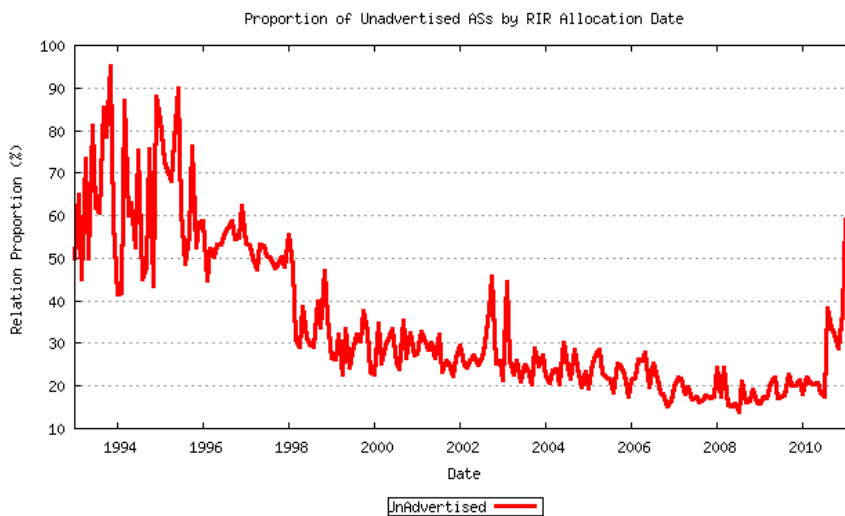
Figure 15 - Advertised / Unadvertised Ratio Series
