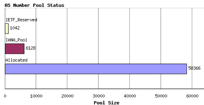
Figure 1 - AS Number Pool Status
