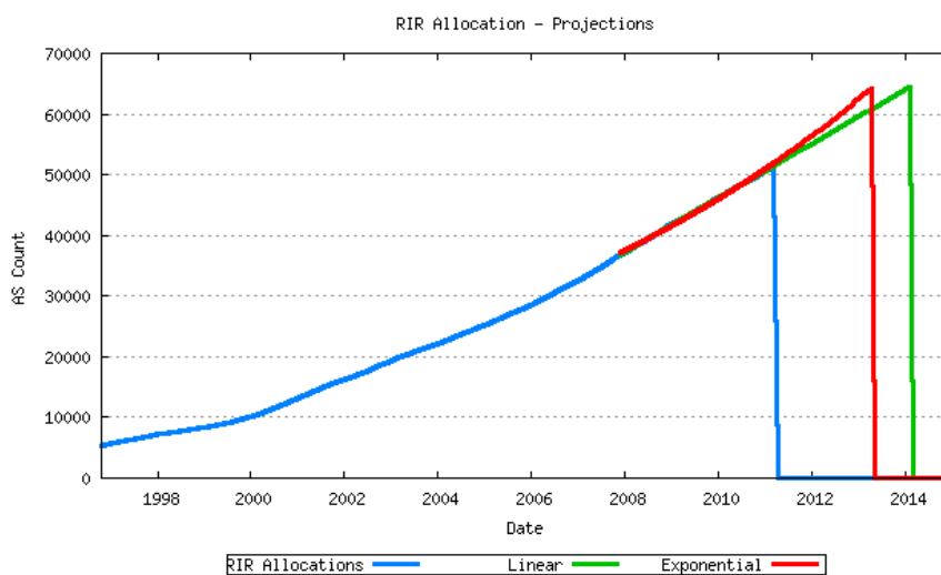
Figure 19 - RIR Assignment projection
