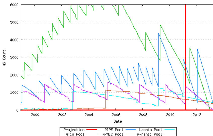
Figure 28 - RIR Pool size - projection
