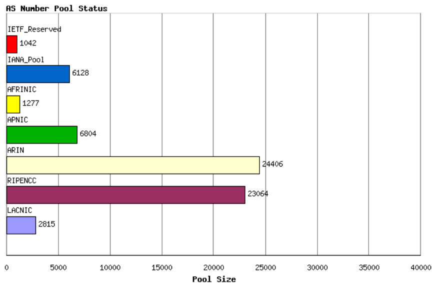
Figure 2 - AS allocations to RIRs
