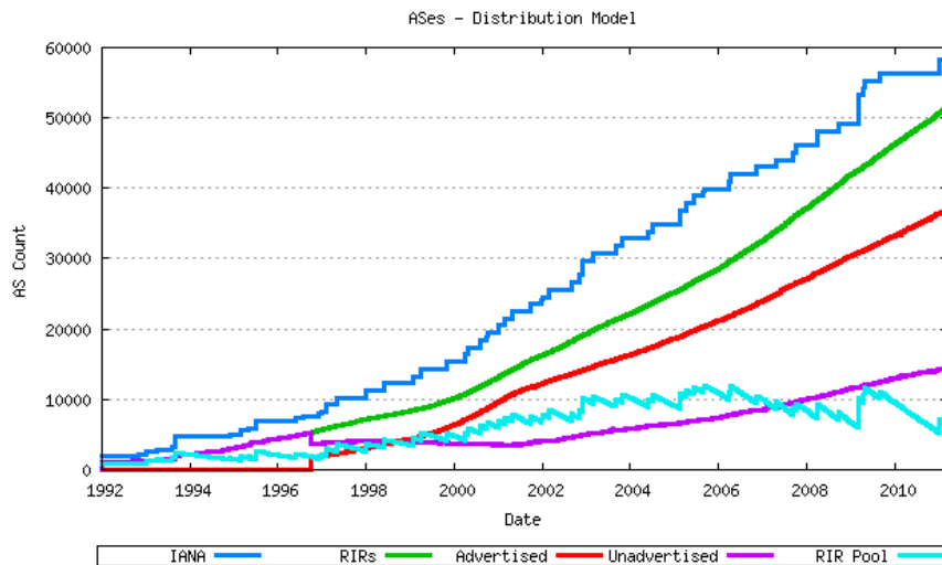
Figure 17 - AS Allocation and Assignment Series
