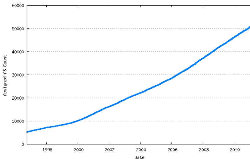
Figure 8 - Cumulative RIR AS assignments
