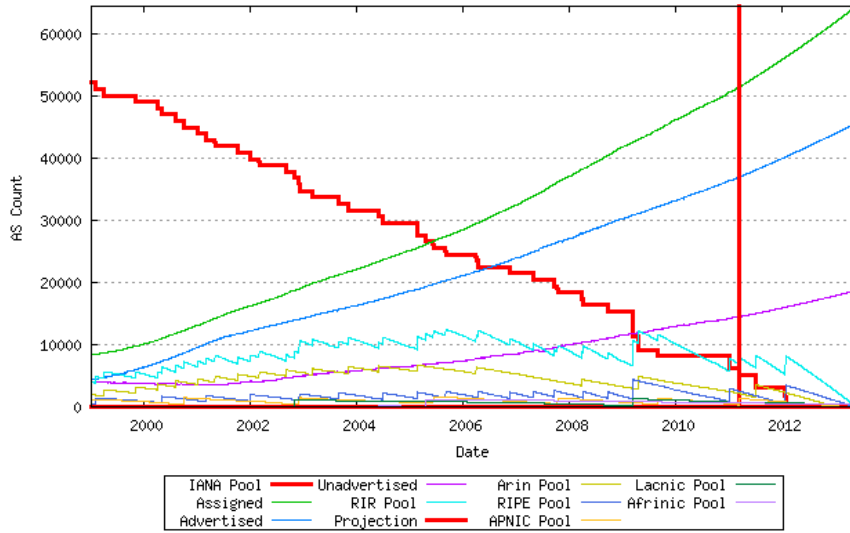
Figure 29 - Predictive model of 2-Byte AS Number consumption
