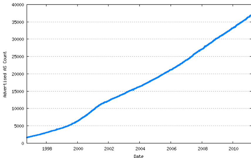
Figure 11 - Advertised AS Count
