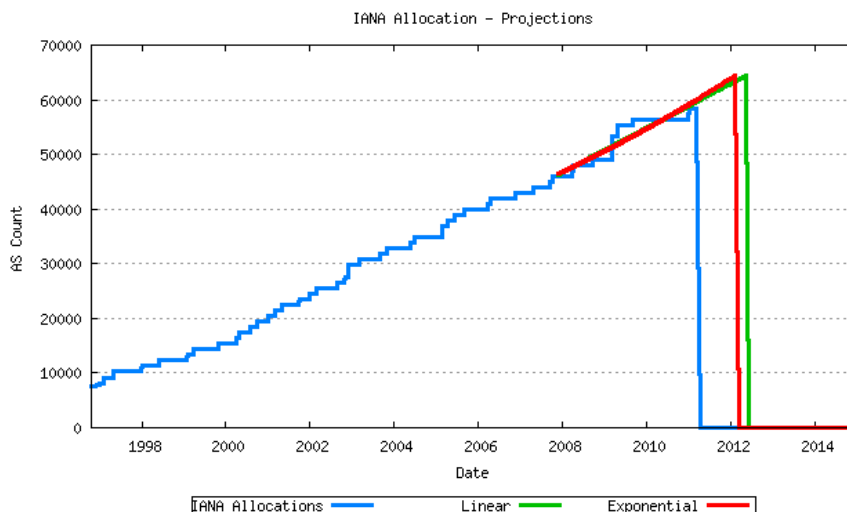
Figure 18 - IANA Allocation projection
