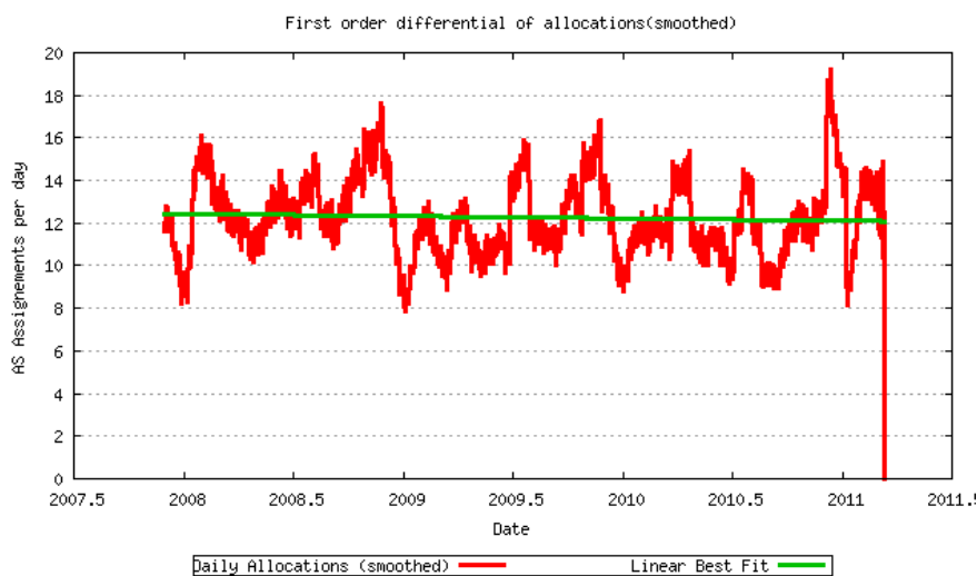
Figure 26 - First order differential of allocation rate
