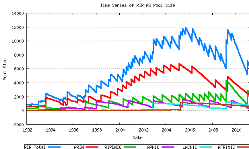
Figure 10 - RIR AS Number Pool size
