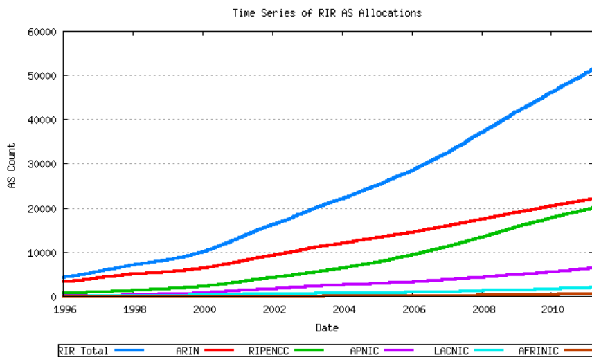
Figure 9 - Cumulative RIR AS assignments per RIR
