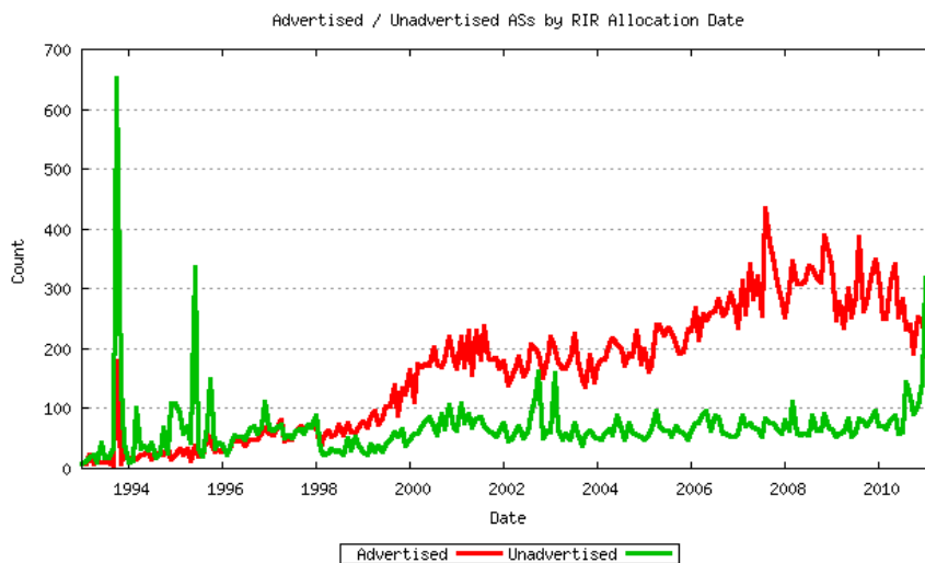
Figure 14 - Advertised / Unadvertised Assignment Series
