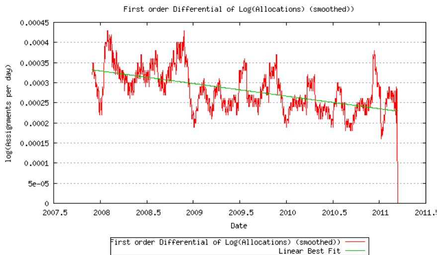
Figure 27 - First order differential of log(allocation rate)
