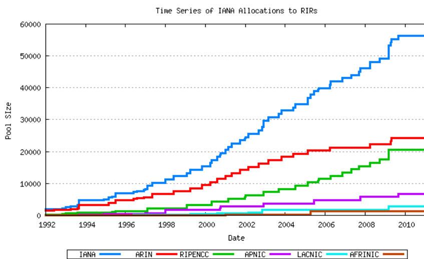
Figure 7 - Cumulative IANA AS block allocations per RIR
