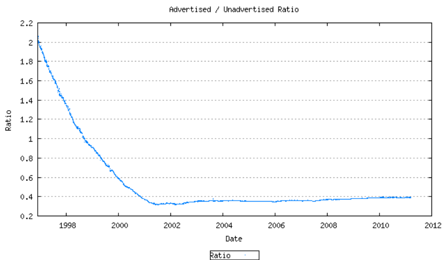
Figure 13 - Advertised / Unadvertised AS Count
