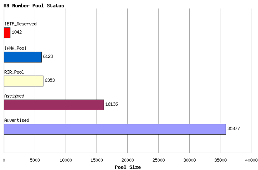
Figure 3 - AS Pools by State
