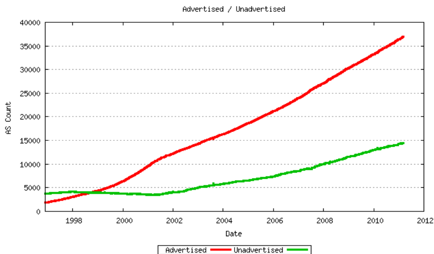
Figure 12 - Advertised / Unadvertised AS Count
