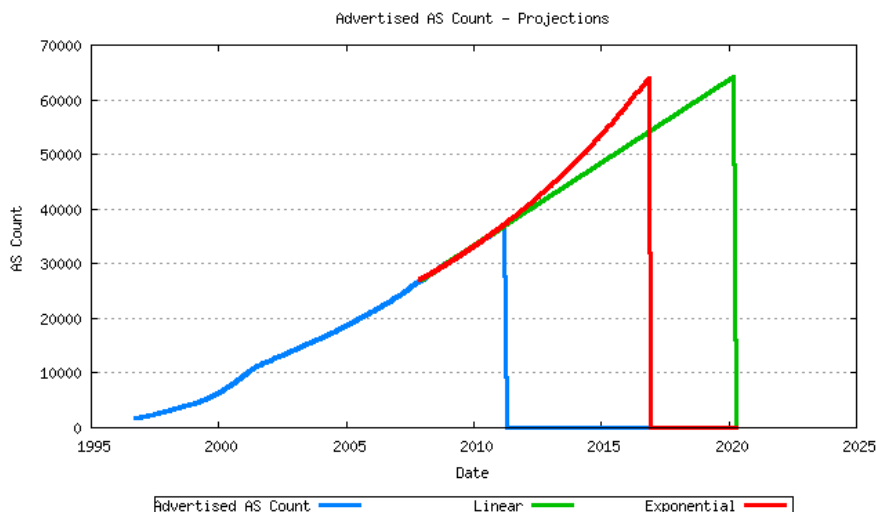
Figure 21 - RIR Assignment projection
