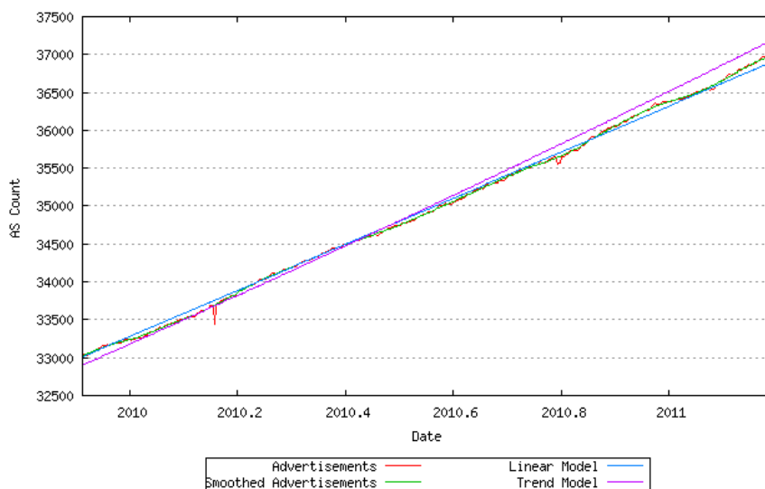
Figure 24 - Allocation Rate - linear and exponential trend best fit
