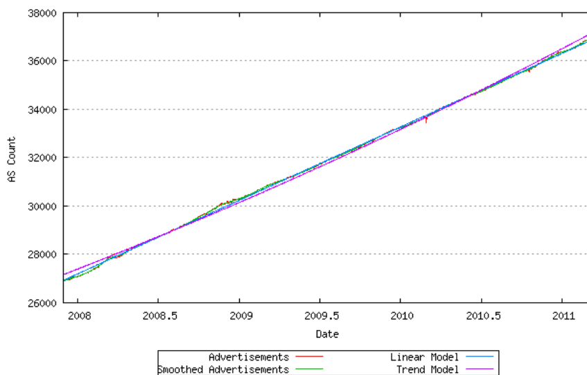
Figure 23 - Allocation Rate - linear and exponential trend best fit
